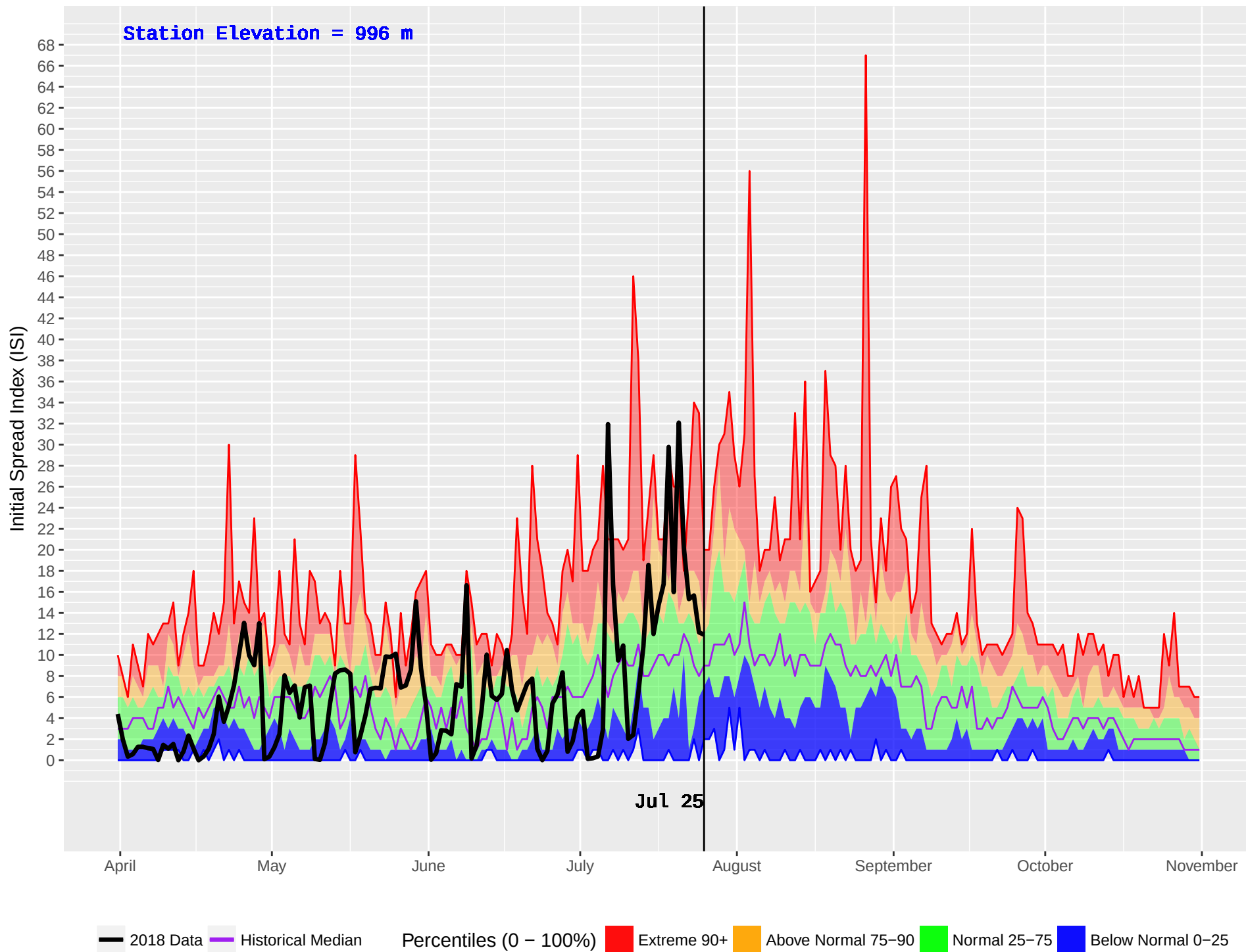
CRANBROOK FS (426) : Historical (2001–2016) and Current (2018) Noon Initial Spread Index (ISI)
