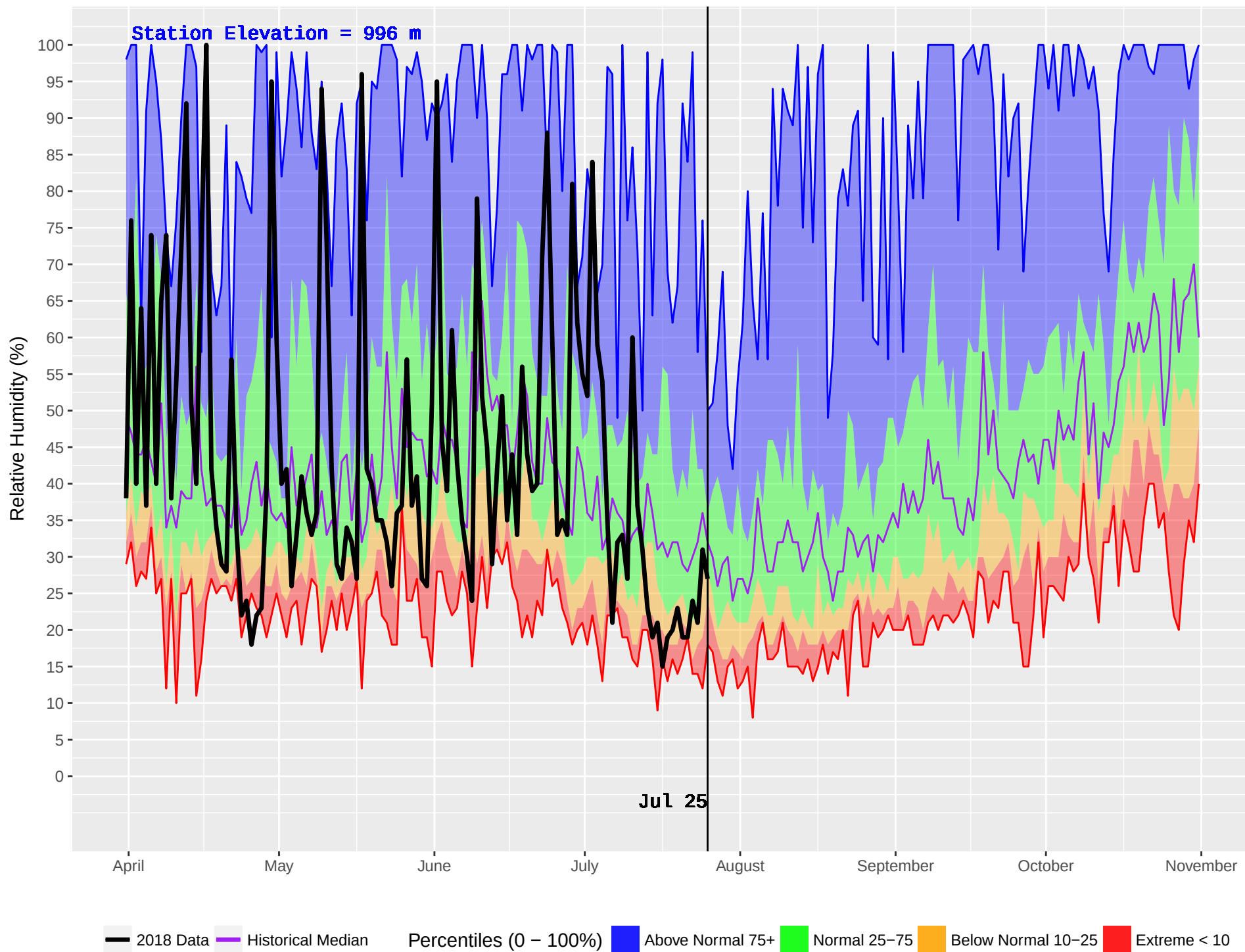
CRANBROOK FS (426) : Historical (2001–2016) and Current (2018) Noon Relative Humidity
